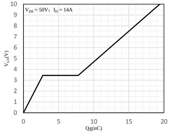
Fig 8 Gate-Charge Characteristics
