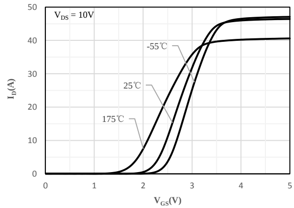
Fig 8 Transfer Characteristics
