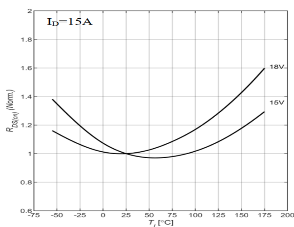
Fig 6 Normalized On-Resistance vs. Junction Temperature
