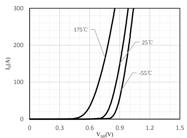
Fig 6 Body-Diode Characteristics
