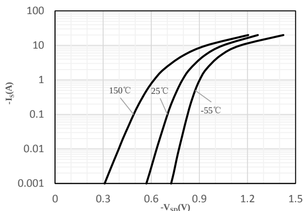
Fig 4 Body-Diode Characteristics
