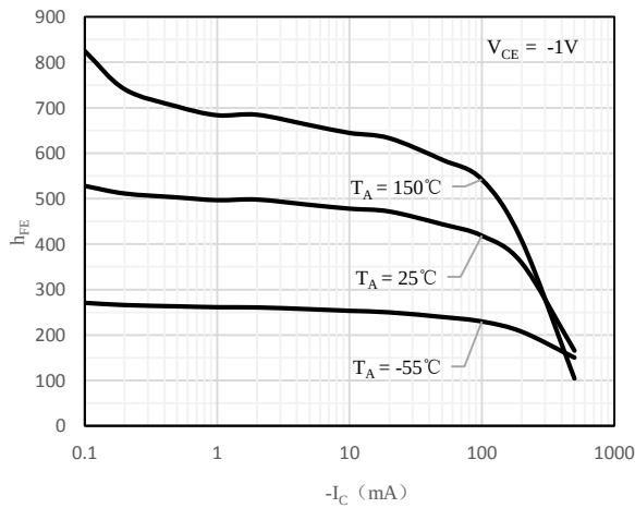
Fig 3 h_{FE} vs. I_C (TBC807-40)
