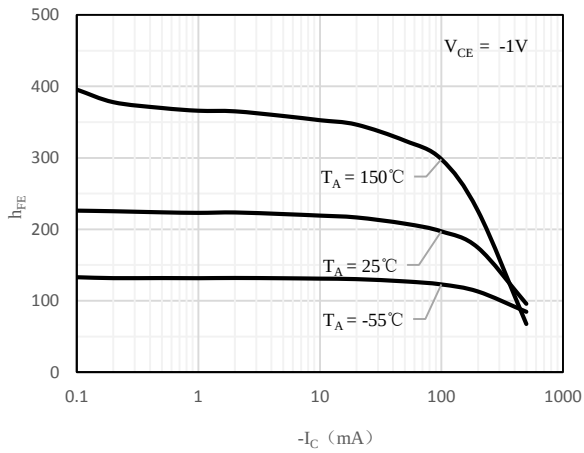
Fig 1 h_{FE} vs. I_C (TBC807-16)
