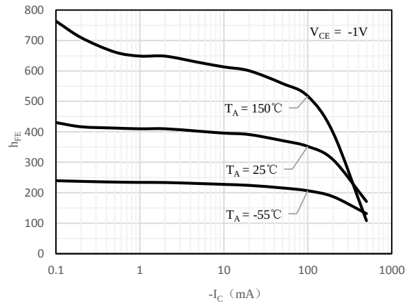
Fig 2 h_{FE} vs. I_C (TBC807-25)
