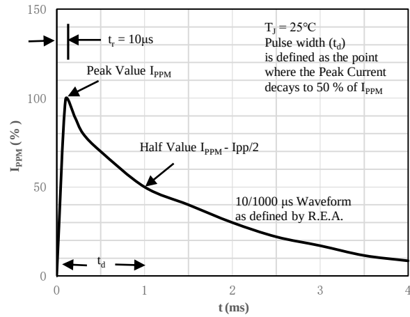
Fig 2 Pulse Waveform
