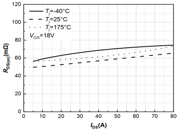
Fig 7 On-Resistance vs. Drain Current
