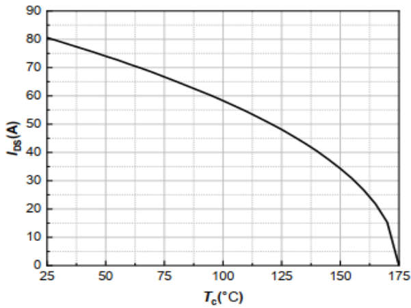
Fig 9 Drain Current
