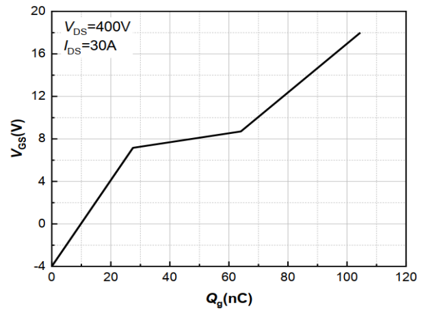
Fig 14 Gate-Charge Characteristics
