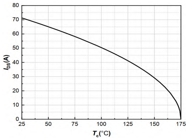
Fig 9 Drain Current
