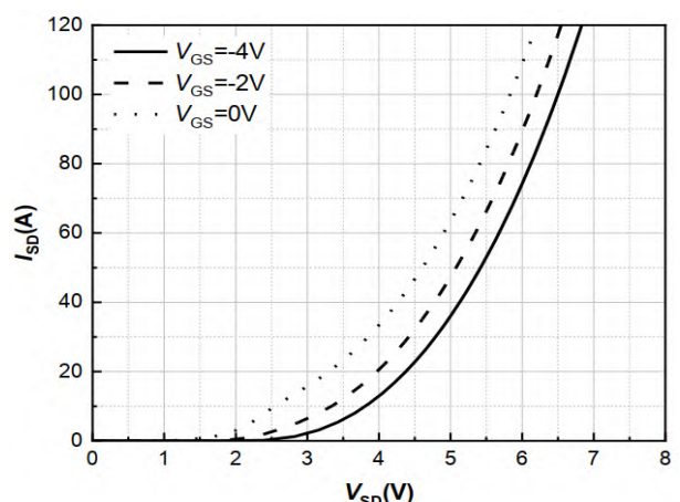
Fig 12 Body-Diode Characteristics ( T_J = 175^\circ\text{C} )
