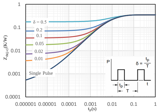
Fig 24 Maximum transient thermal impedance
