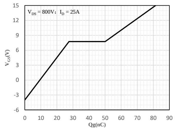
Fig 16 Gate-Charge Characteristics
