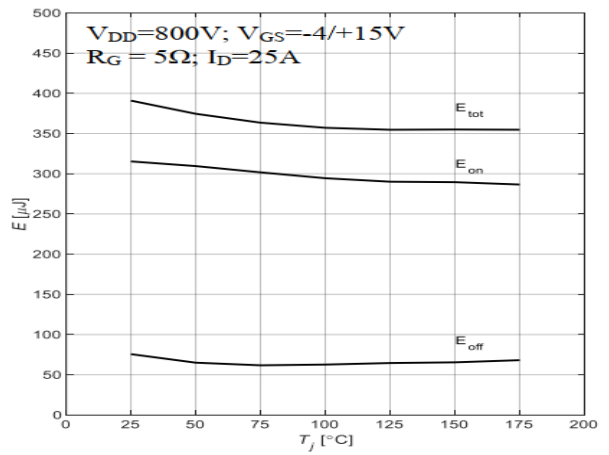
Fig 22 Clamped Inductive Switching Energy vs. T_J
