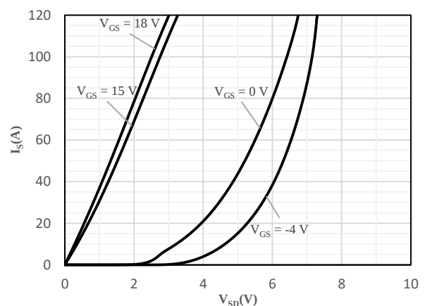
Fig 12 Body-Diode Characteristics ( T_J = -55^\circ\text{C} )
