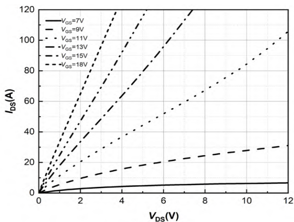
Fig 2 Typical Output Characteristics ( T_j = -40^\circ\text{C} )
