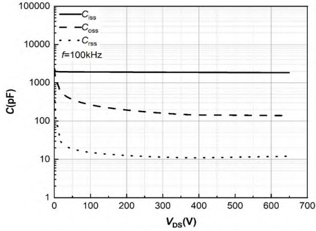
Fig 13 Capacitance Characteristics
