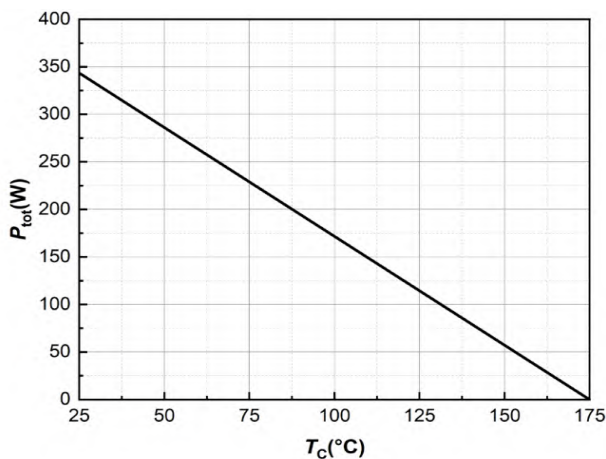
Fig 1 Power Dissipation
