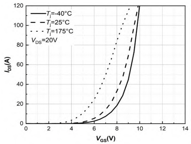
Fig 8 Transfer Characteristics
