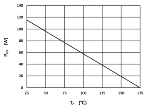
Fig 7 Power Derating
