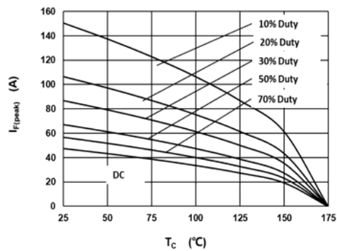
Fig 5 Current Derating
