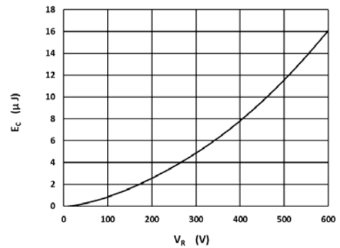
Fig 6 Typical Capacitance Stored Energy
