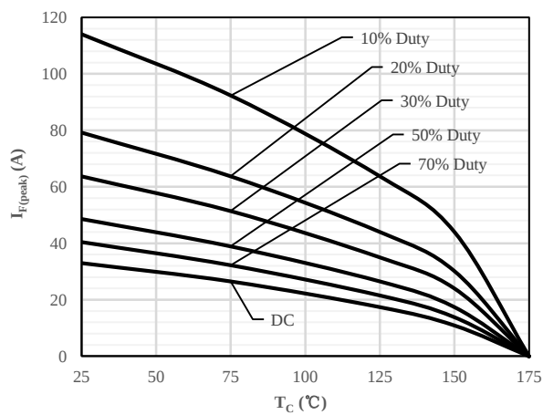
Fig 5 Current Derating
