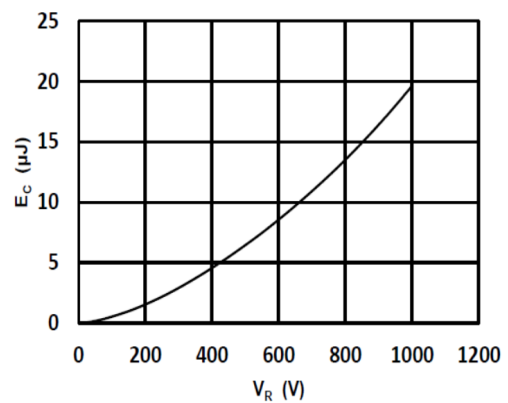
Fig 6 Typical Capacitance Stored Energy
