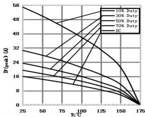
Fig 5 Current Derating
