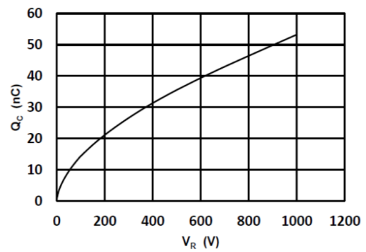
Fig 4 Reverse Charge vs. Reverse Voltage
