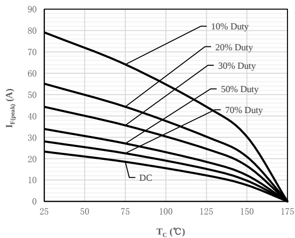
Fig 5 Current Derating
