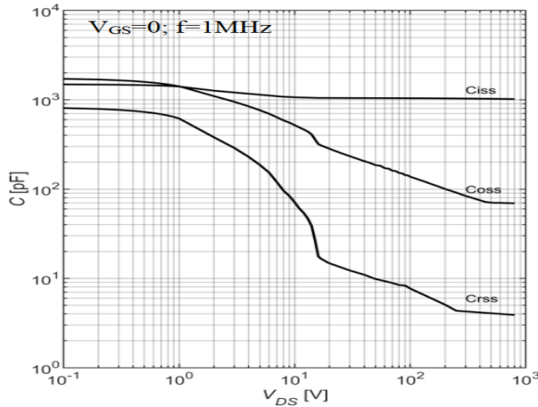
Fig 13 Capacitance Characteristics
