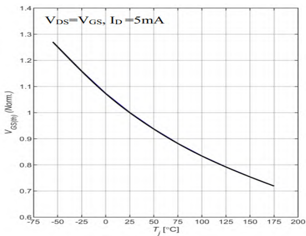
Fig 5 Normalized V_{GS(th)} vs. Junction Temperature
