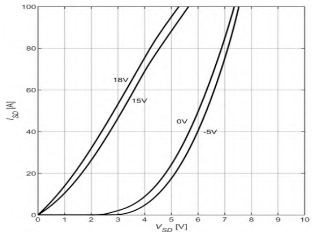
Fig 10 Body-Diode Characteristics ( T_J = -55°C )
