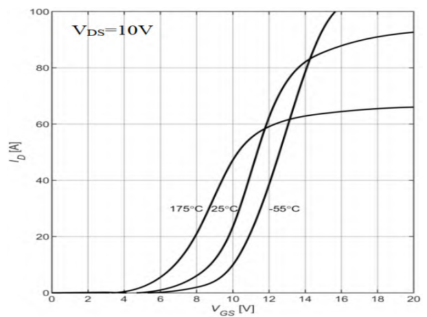
Fig 8 Transfer Characteristics
