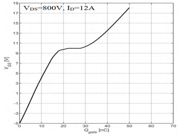
Fig 14 Gate-Charge Characteristics
