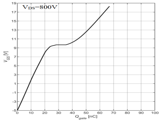
Fig 14 Gate-Charge Characteristics
