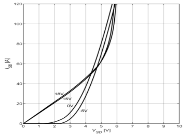
Fig 12 Body-Diode Characteristics ( T_J = 175^\circ C )
