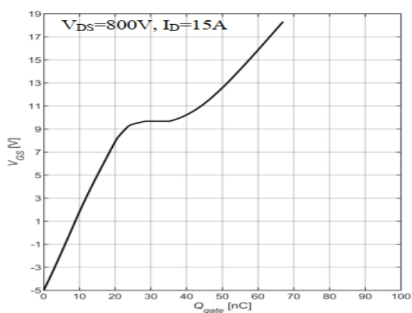
Fig 14 Gate-Charge Characteristics
