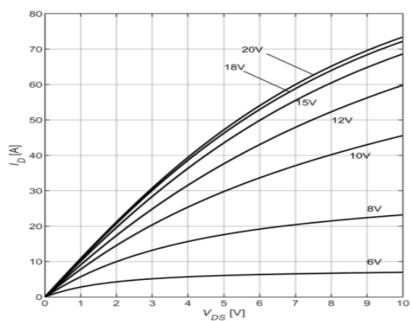
Fig 4 Typical Output Characteristics ( T_J = 175^\circ\text{C} )
