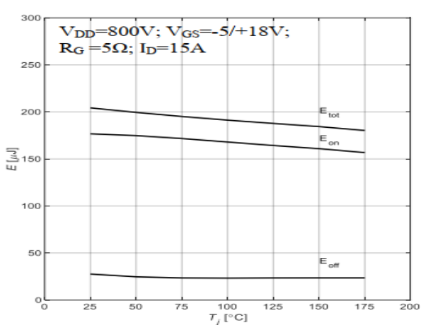
Fig 18 Clamped Inductive Switching Energy vs. Junction Temperature
