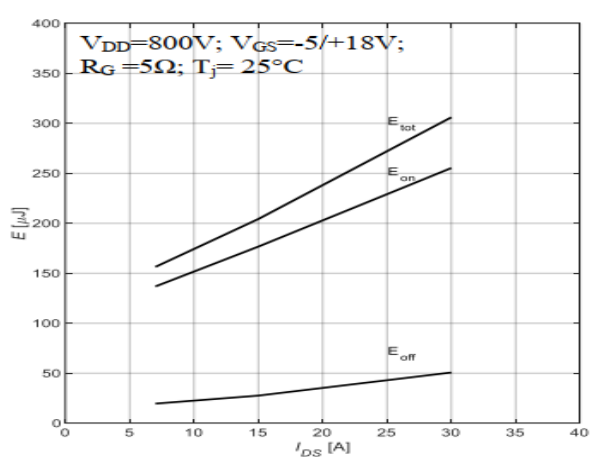
Fig 16 Clamped Inductive Switching Energy vs. Drain Current
