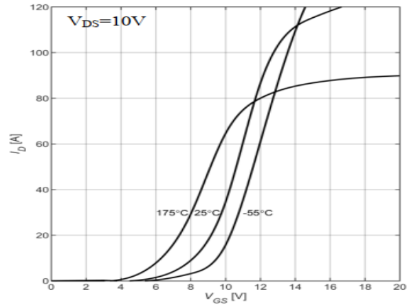
Fig 8 Transfer Characteristics
