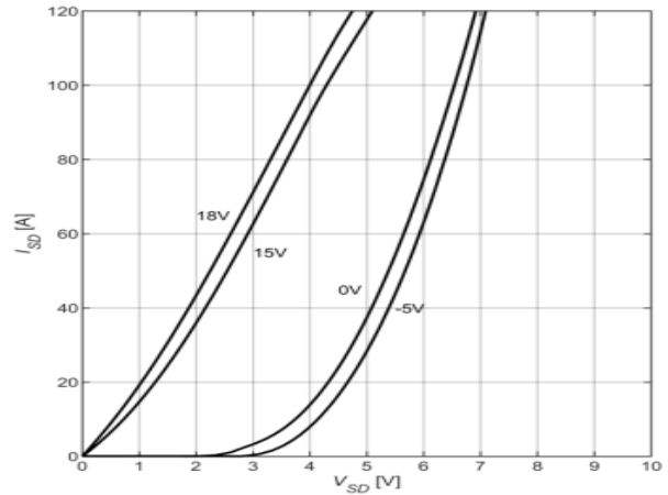
Fig 10 Body-Diode Characteristics ( T_J = -55^\circ C )
