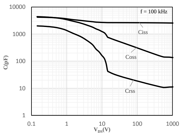
Fig 15 Capacitance Characteristics
