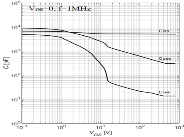
Fig 13 Capacitance Characteristics
