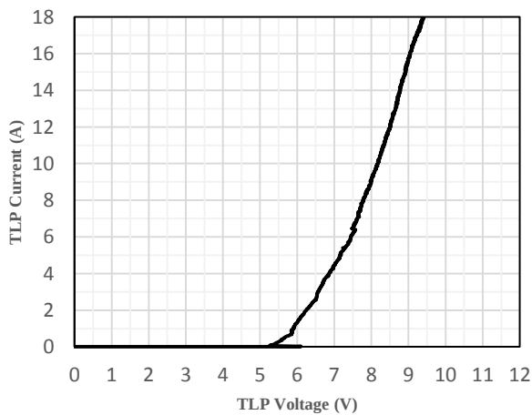
Fig 5 TLP Measurement
