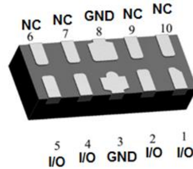
DFN2510-10L
