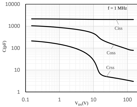
Fig 9 Capacitance Characteristics
