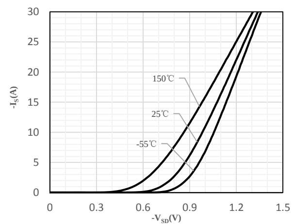
Fig 6 Body-Diode Characteristics
