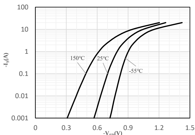
Fig 4 Body-Diode Characteristics
