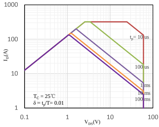
Fig 13 Safe Operation Area
