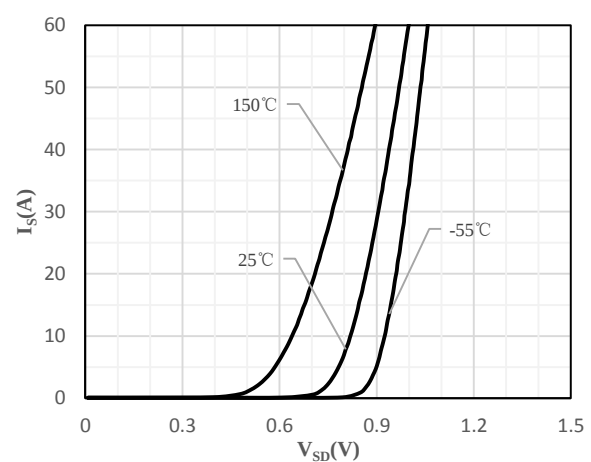
Fig 6 Body-Diode Characteristics
