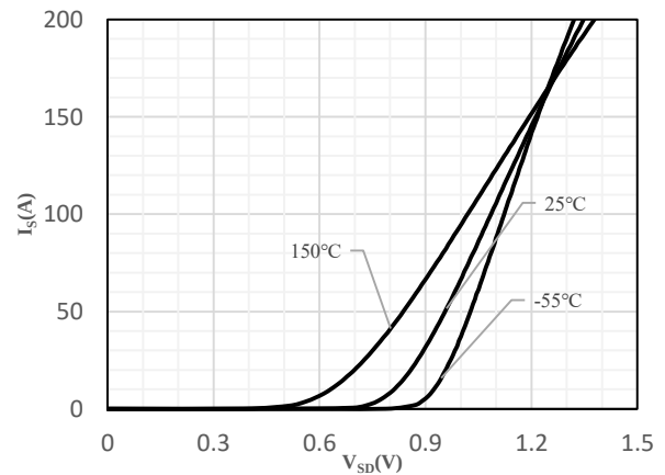
Fig 6 Body-Diode Characteristics
