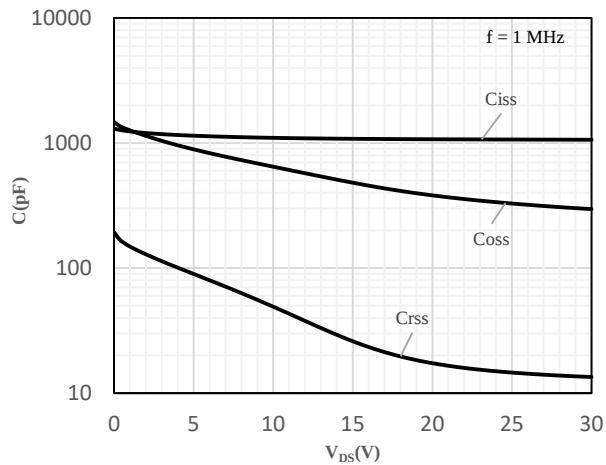
Fig 7 Capacitance Characteristics
