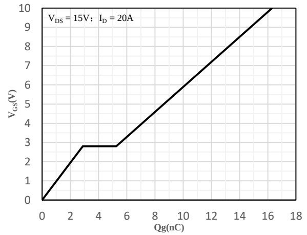
Fig 8 Gate-Charge Characteristics
