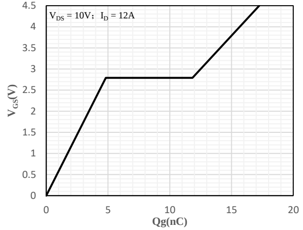
Fig 10 Gate-Charge Characteristics
