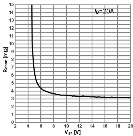
Fig 3 On-Resistance vs. Gate-Source Voltage
