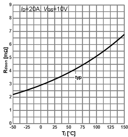
Fig 5 On-Resistance vs. Junction Temperature
