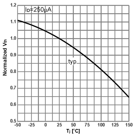
Fig 9 Normalized V_{GS(th)} vs. Junction Temperature
