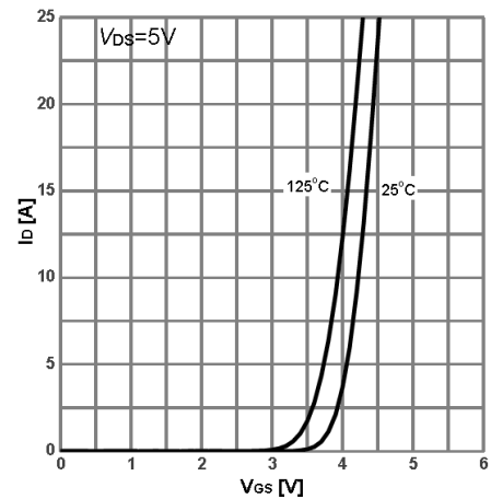
Fig 6 Transfer Characteristics
