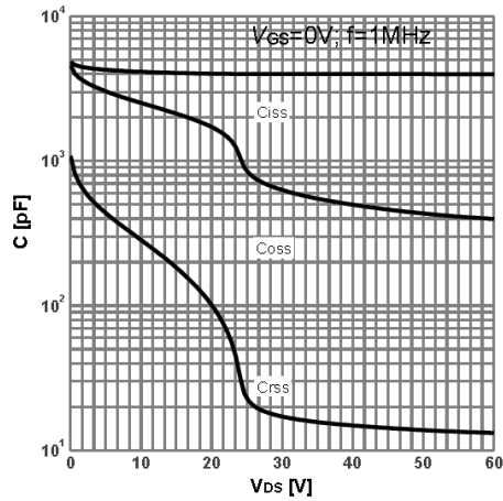
Fig 7 Capacitance Characteristics
