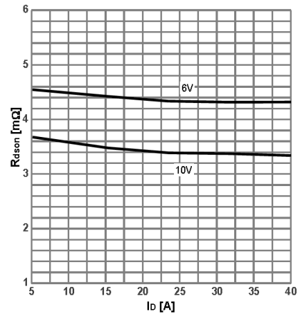
Fig 2 On-Resistance vs. Drain Current and Gate Voltage
