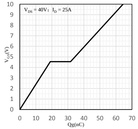
Fig 8 Gate-Charge Characteristics
