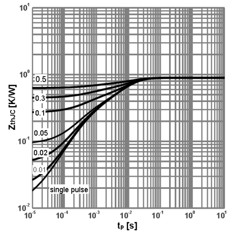
Fig 10 Maximum transient thermal impedance
