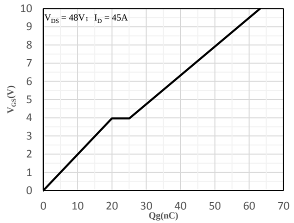
Fig 8 Gate-Charge Characteristics
