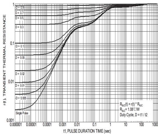
Fig 11 Transient Thermal Resistance
