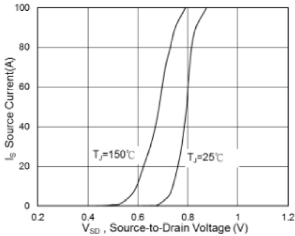
Fig.3 Forward Characteristics of Reverse diode
