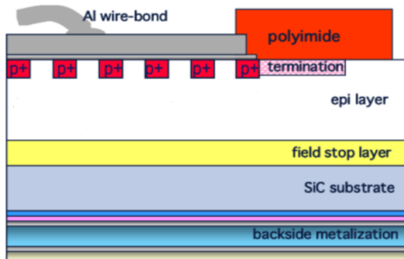
SiC JBS Die Cross-section
